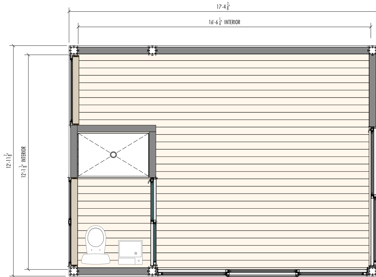
1 K4 12' EXTENDED BATH 226 SF
