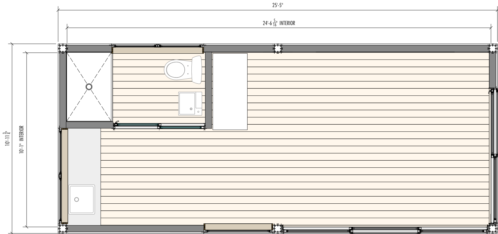
1 K6 10FT BATH + KITCHENETTE 280 SF
