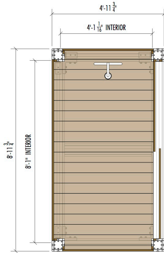
1 Kbath OUTDOOR SHOWER 4x8 45 SF
