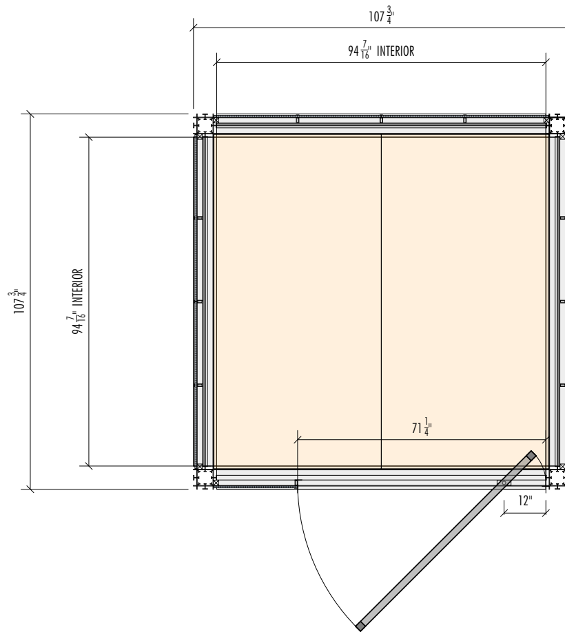
1 K3 CUBE 8X8 81 SF
