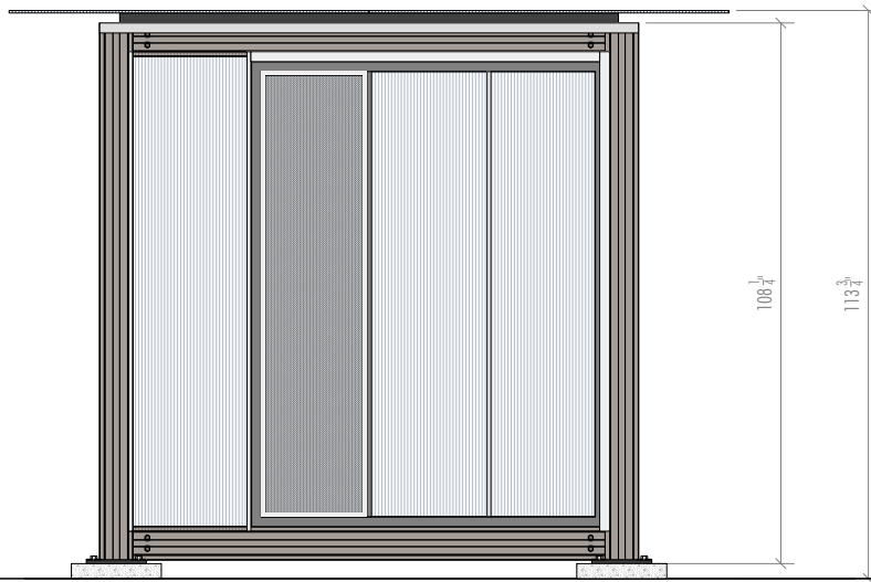
1 FRONT EXTERIOR ELEVATION SCALE 1/2" = 1'-0"
