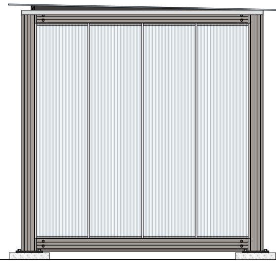
2 BACK & SIDES EXTERIOR ELEVATION SCALE 1/2" = 1'-0"
