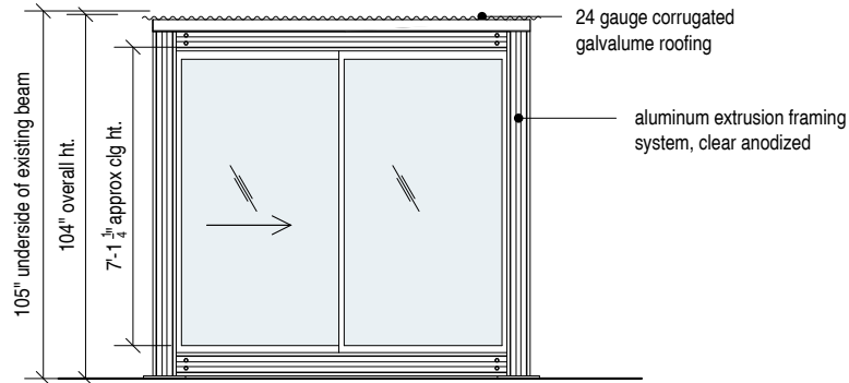
2 front elevation scale: 1/4" = 1'-0"
