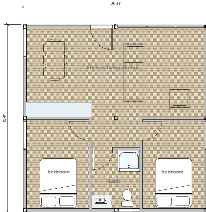
k6+k6 (square plan)
