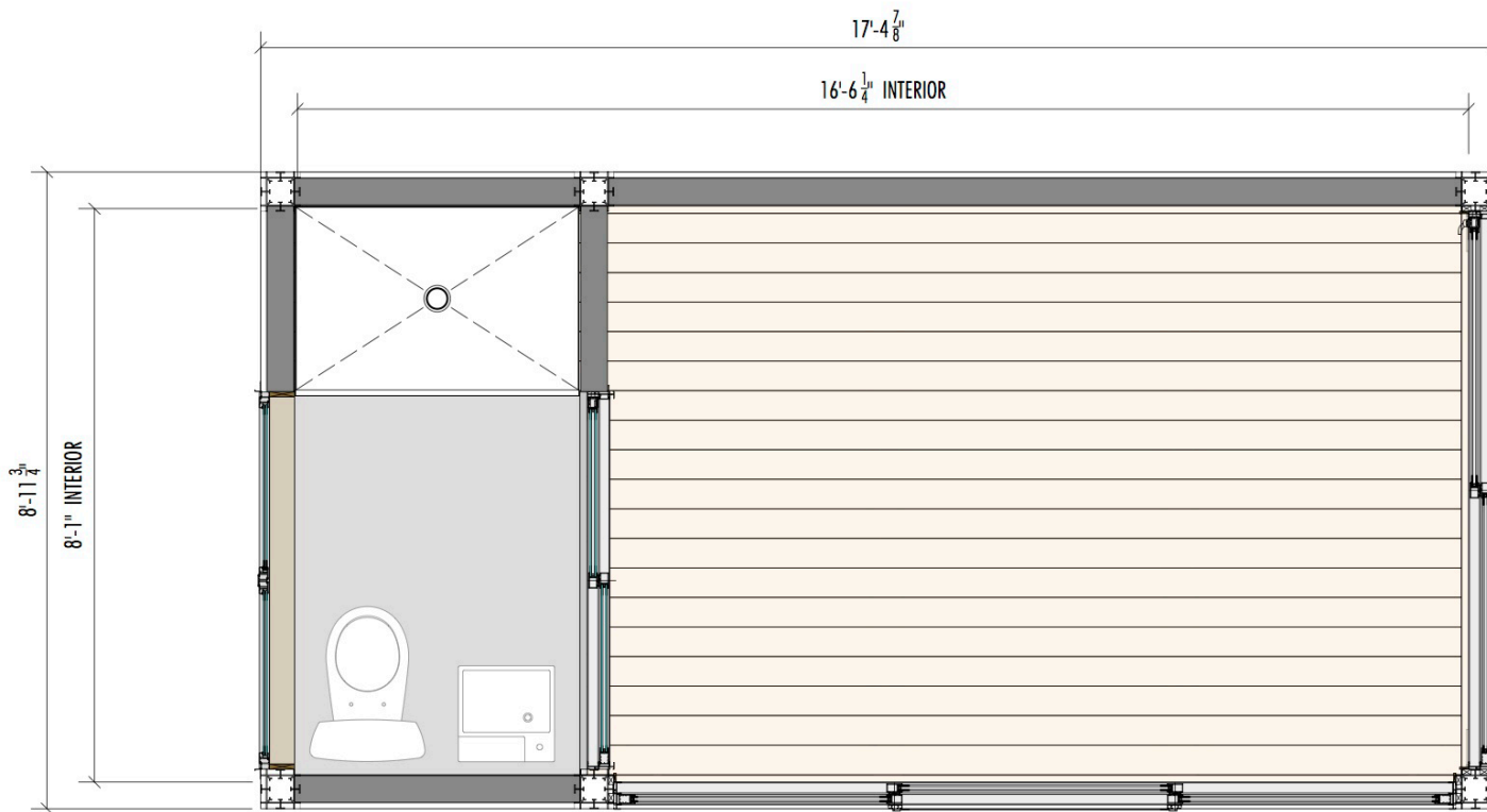
1 K4 BATH : NARROW (8FT) 157 SF
