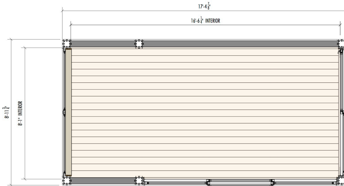
1 K4 BASIC : NARROW (8FT) 157 SF
