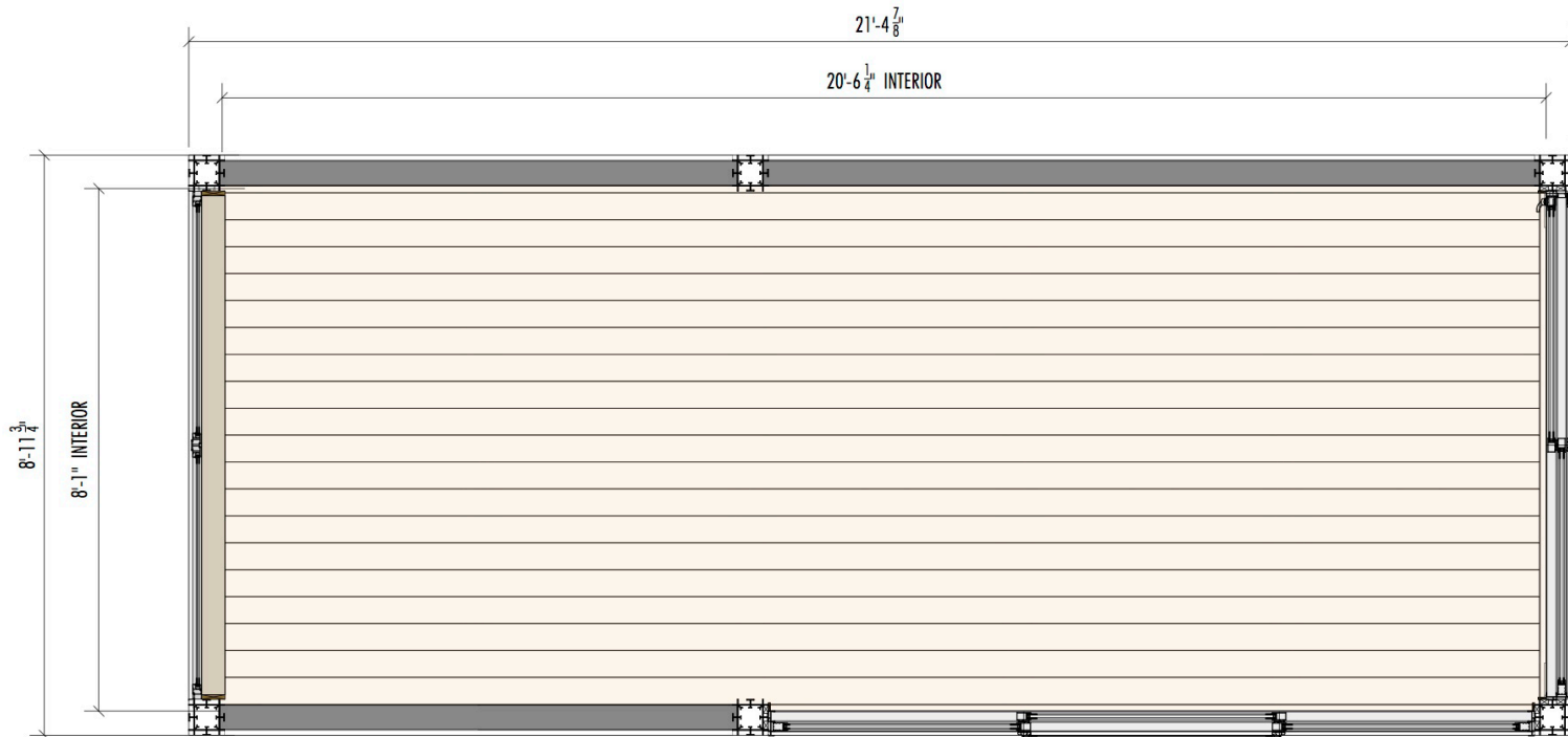
1 K5 BASIC : NARROW (8FT) 192 SF
