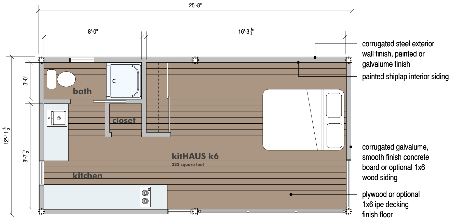
kitHAUS k6 floor plan
